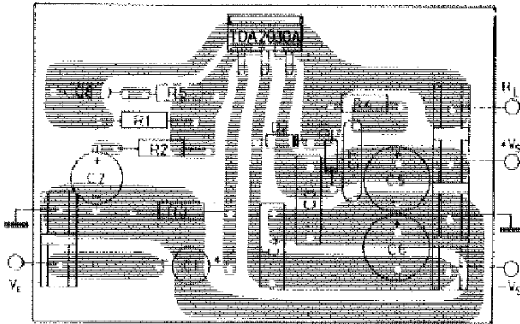
Figure 15 : P.C. Board and Component Layout for the Circuit of Figure 14 (1:1 scale)
