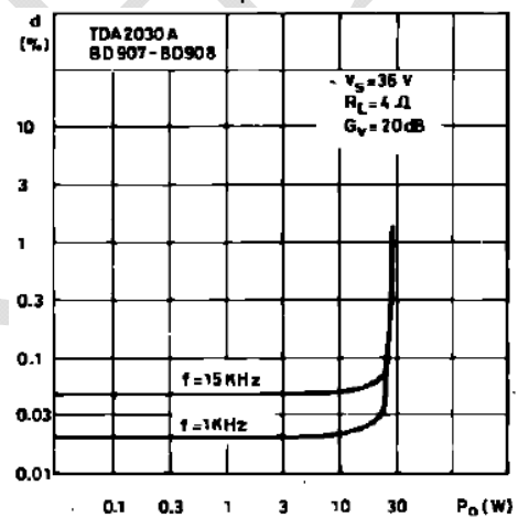
Figure 9 : Total Harmonic Distortion versus Output Power
