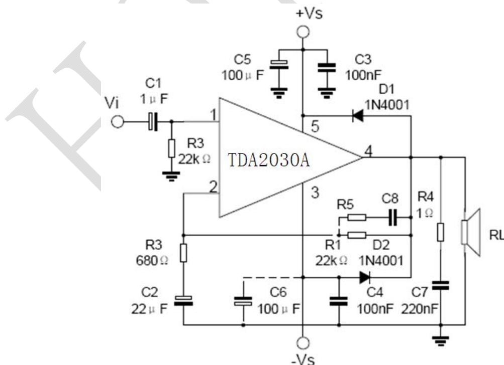
Figure14: Typical Amplifier with Split Power Supply
