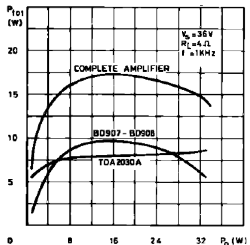
Figure 11 : Power Dissipation versus Output Power
