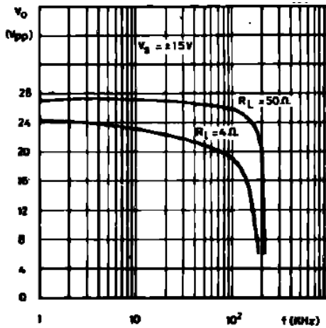
Figure 6 : Large Signal Frequency Response Dissipation
