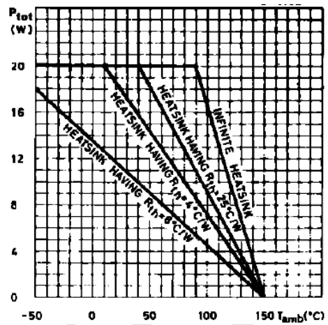
Figure 7 : Maximum Allowable Power versus Ambient Temperature
