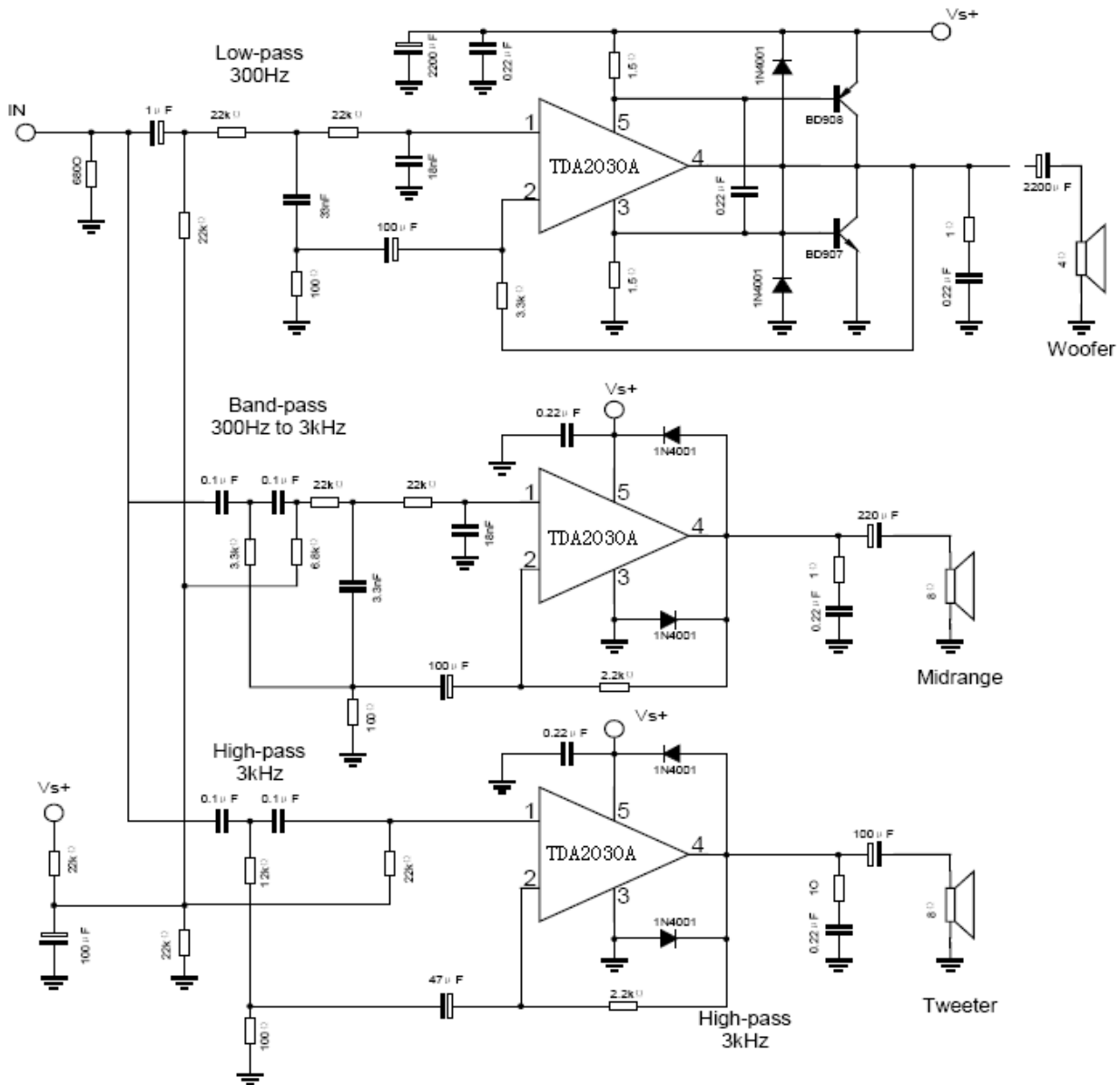
Figure 20 : 3 Way 60W Active Loudspeaker System(VS=36V)
