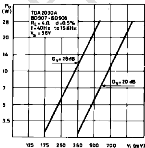
Figure 10 : Output Power versus Input Level
