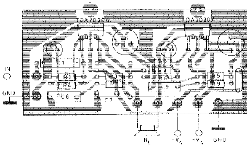
Figure 17 : P.C.Board and Component Layout for the Circuit of Figure16(1:1 scale)
