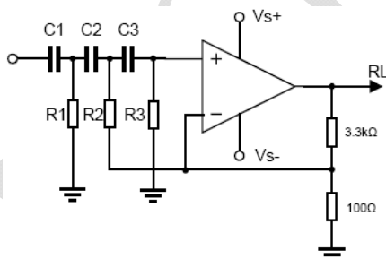
Figure 19 : Active Power Filter.
