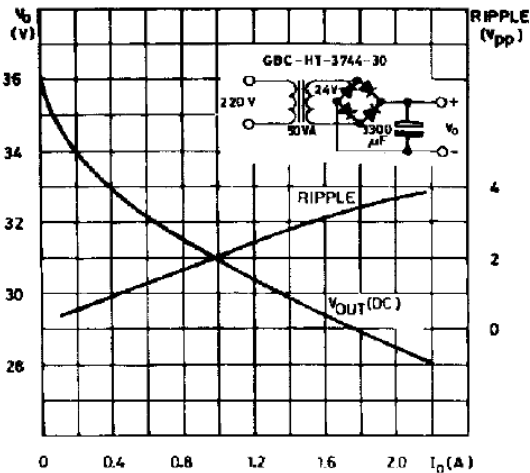
Figure 27 : DC Characteristics of 50W Non-regulated Supply
