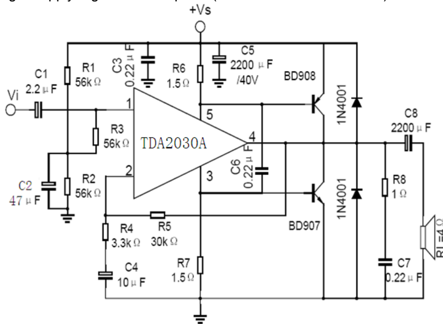
Figure 12 : Single Supply High Power Amplifier (TDA2030A+BD907/BD908)
