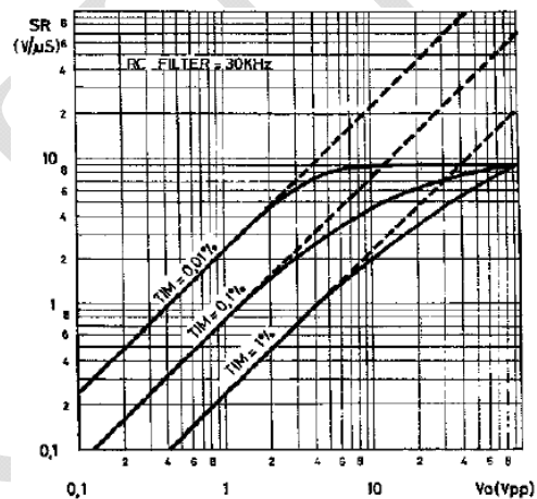
Figure 26: TIM Design Diagram (fc = 30kHz)
