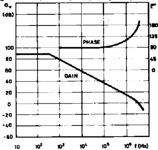
Figure 2: Open Loop-frequency Response
