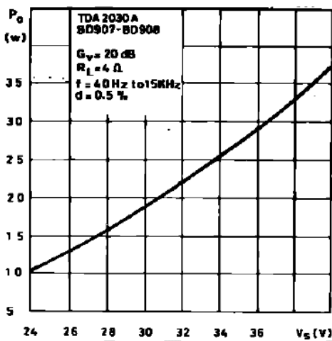
Figure 8 : Output Power versus Supply Voltage
