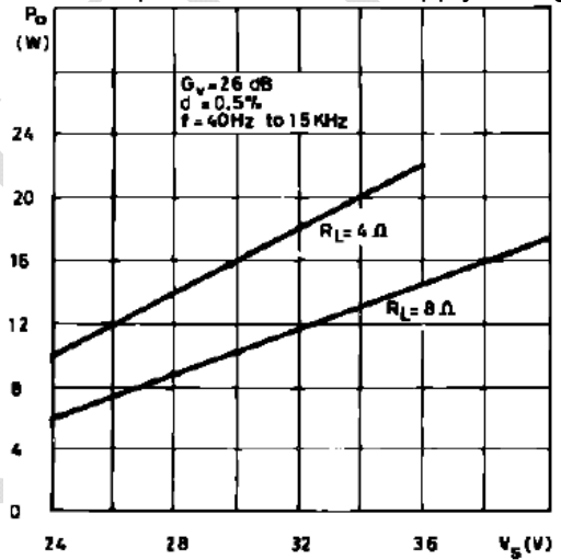
Figure 3: Output Power versus Supply Voltage
