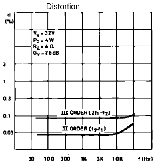
Figure 5: Two Tone CCIF Intremodulation Distortion
