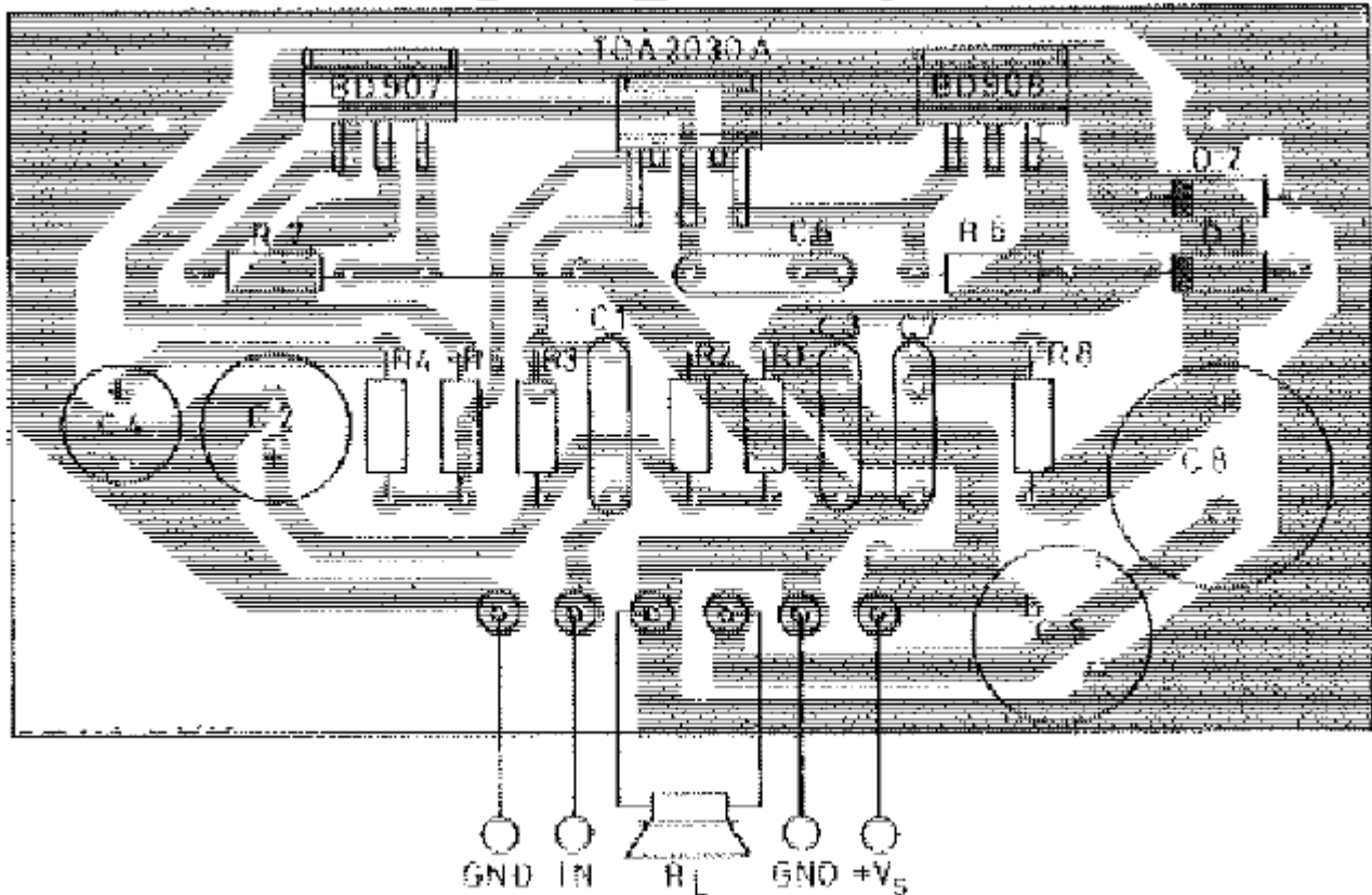
Figure 13 : P.C. Board and Component Layout for the Circuit of Figure 12 (1:1 scale)
