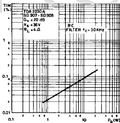
Figure 25 : TIM Distortion versus Output Power
