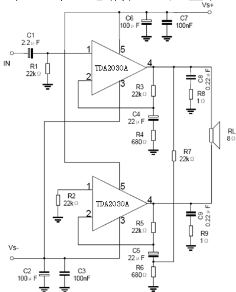
Figure 16 : Bridge Amplifier with Split Power Supply (PO = 34W, VS = 16V)
